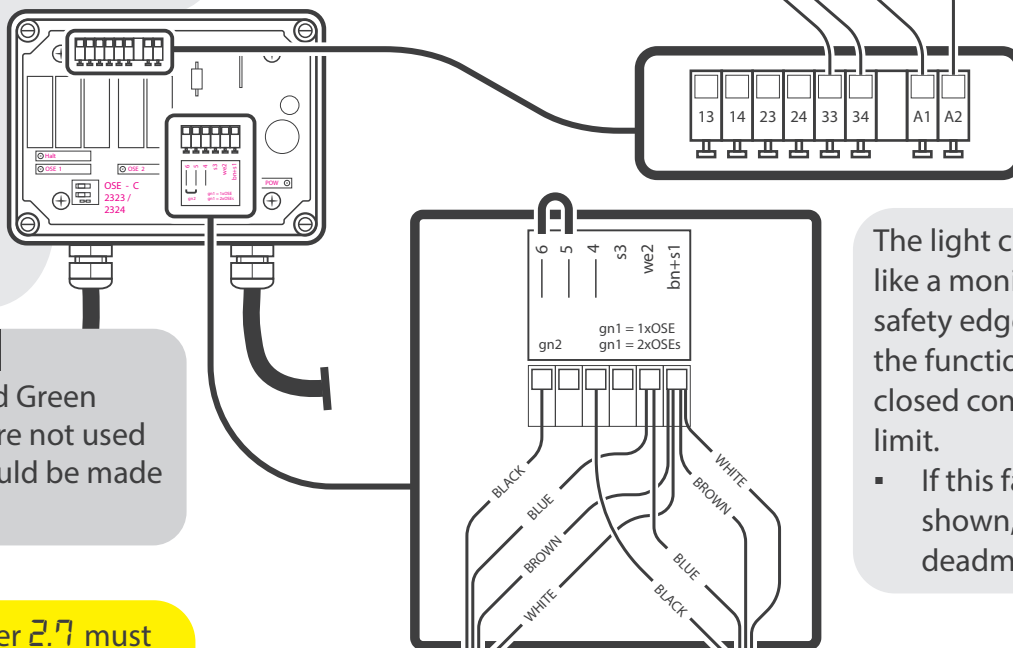
Light Curtain 2
